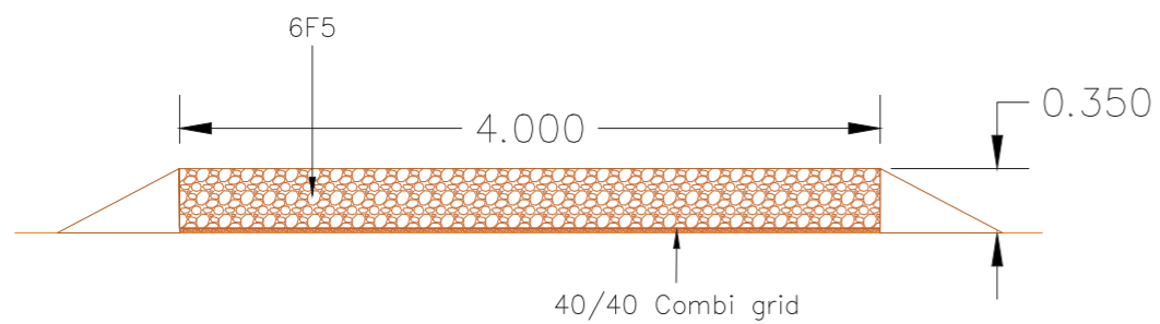
Alternative No-dig (Non-intrusive) access track
