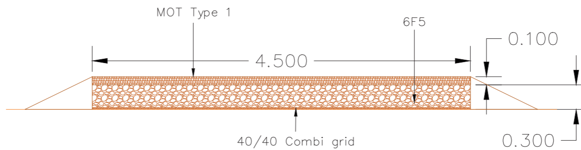
Alternative No-dig (Non-intrusive) DNO access track
