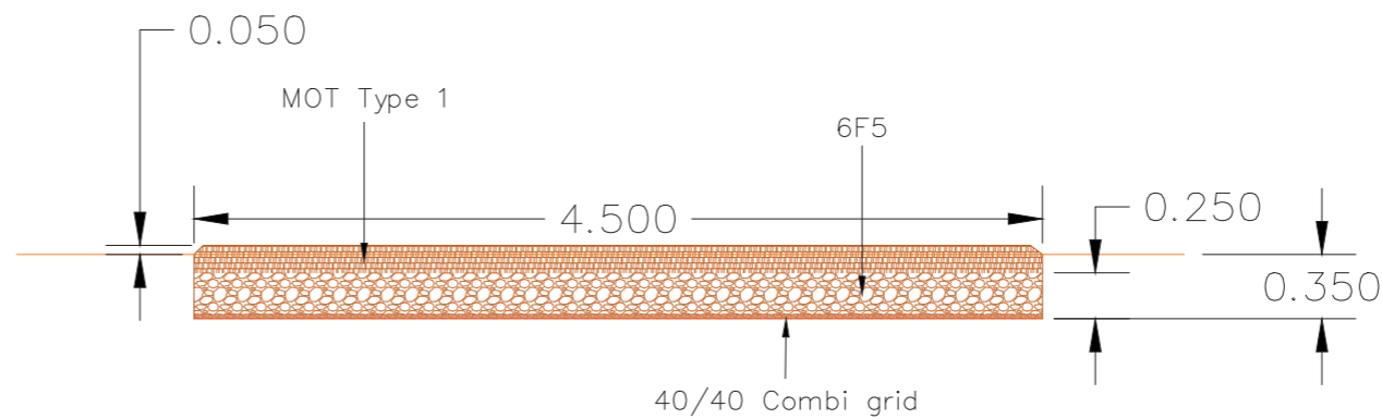
Typical DNO access track cross section
